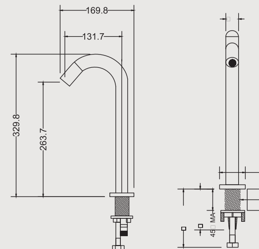
TALL BODY SENSOR TAP IMMACULA CAT CODE: F240006CP | MRP: 13590
