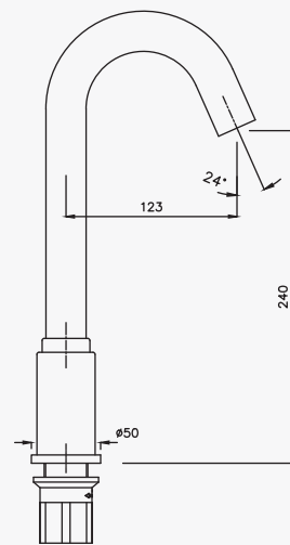
TALL PILLAR SENSOR FLORA CAT CODE: F240009CP | MRP: 9590
